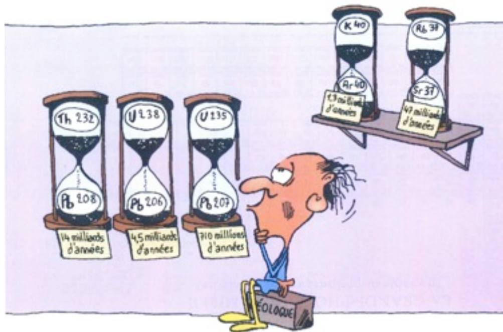
The constant decay time of the disease can be used as a clock.
